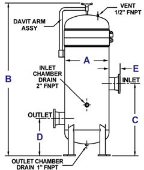
Typical Dome Top Configuration
